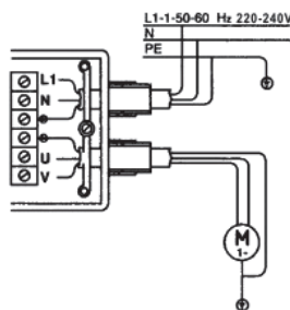
Wiring diagram for connection of single-phase 220V pumps up to 3.0 Kw.
