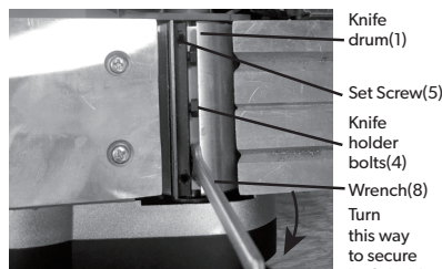
Figure F: Tightening the knife holder
